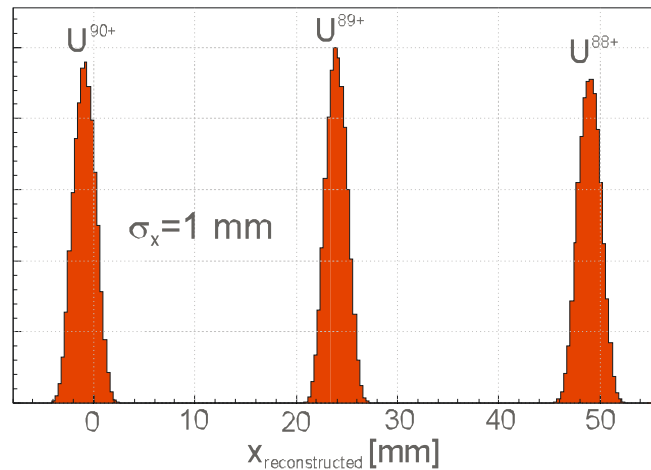
Figure B.24: Resolution obtained with tracking detectors in front and behind the third dipole. Peaks are broadened due to straggling in detector and housing material. From the observed width, a resolving power of R=1100 is derived.
