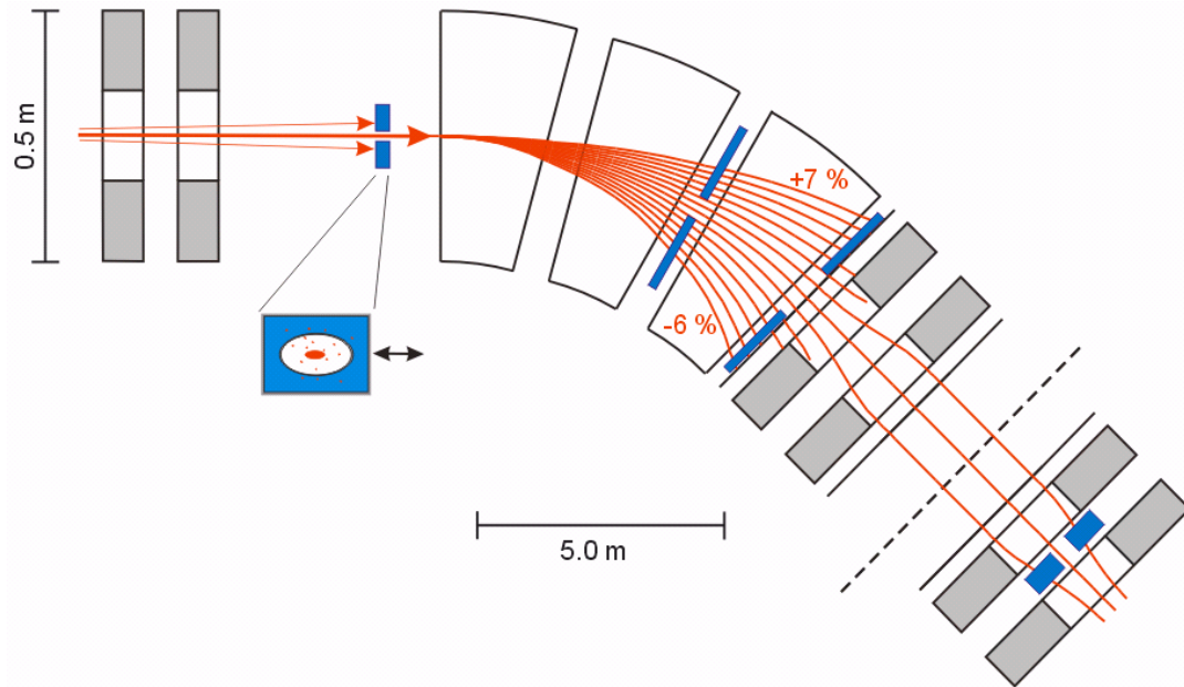
Figure B.22: Trajectories calculated for ions of different magnetic rigidity in the first 45° bending section behind the NESR internal target. The quadrupole doublet behind the target, followed by three dipole magnets and four more quadrupole magnets are shown. Trajectories in red are displayed for beam-like reaction products hitting the tagging detector in front of the dipole and in steps of 1% relative difference in magnetic rigidity in the dipoles. The detector positions are marked in blue color. The mid plane of the full 90° bending section is indicated (dashed line).
