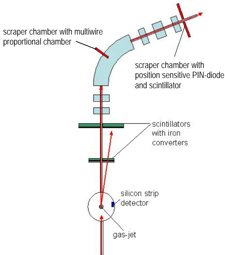
Figure D.2: Experimental set-up for test experiment at the ESR.
