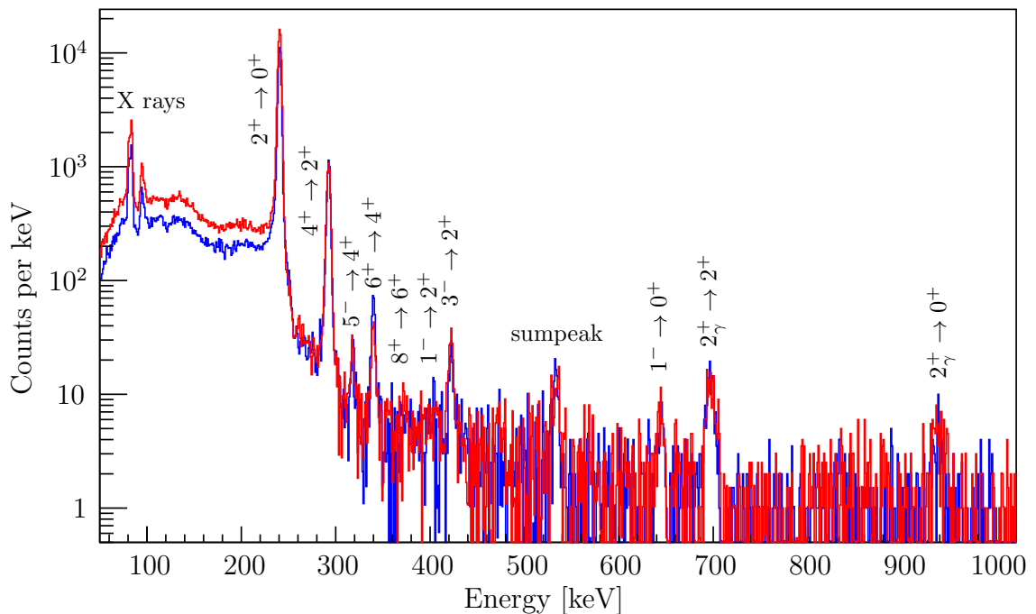
Figure 4.10: Comparison of high centre of mass (CoM) scattering angular range (blue) and low CoM angular range (red) with the ^{220}\text{Rn} beam on ^{120}\text{Sn} target. As with the change of target Z , the change in angle yields different cross sections for exciting states with the variation in intensities reflecting this.
