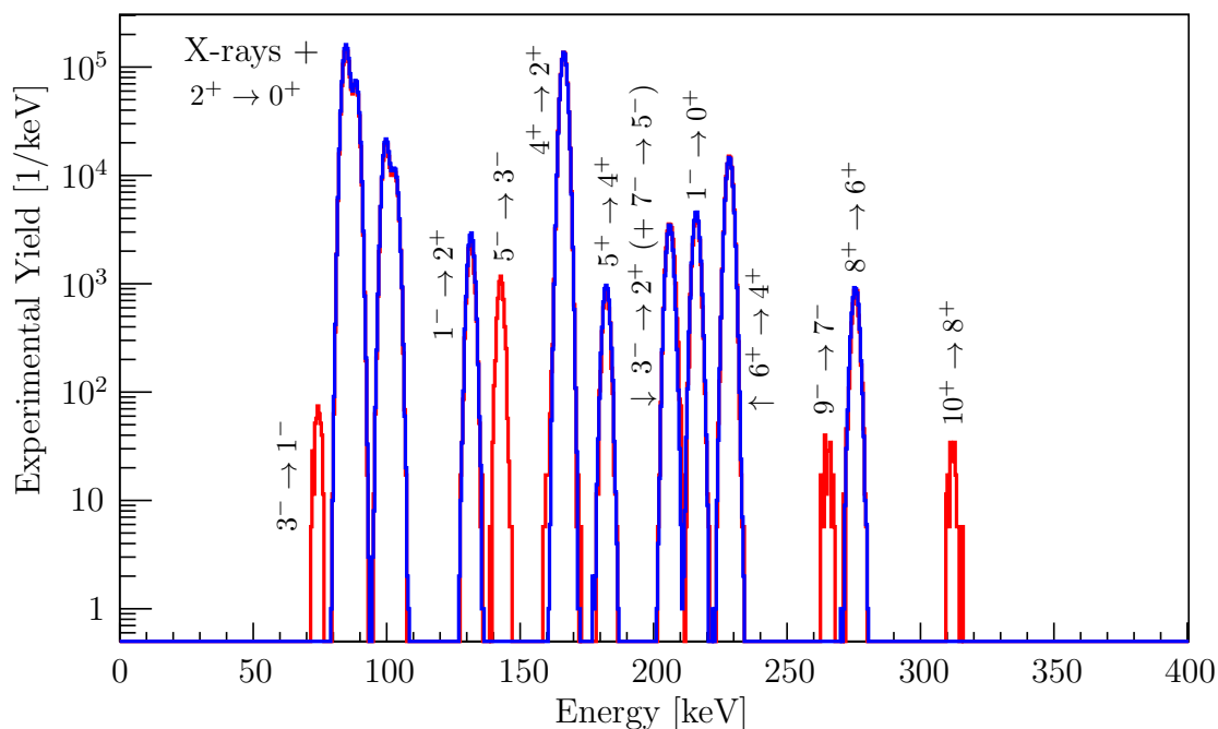
Figure 6.6: Comparison of simulated \gamma -ray yields in ^{224}\text{Ra} , experiment 2 (see Table 5.1), calculated using the measured matrix elements from Table 5.6 (red) and the measured experimental yields from Table B.2 (blue). The 5^+ \rightarrow 4^+ transition is unobserved experimentally due to the large Compton background. The simulated yields are normalised to the 4^+ \rightarrow 2^+ transition.
