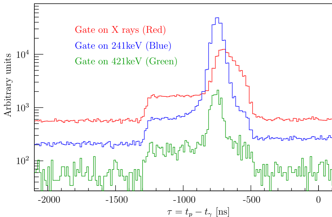
Figure 4.2: Particle- \gamma time difference in the ^{220}\text{Rn} on ^{60}\text{Ni} experiment, gated on the energy range for X rays (red), the 2^+ \rightarrow 0^+ transition at 241 keV (blue) and the 3^- \rightarrow 2^+ transition at 421 keV (green). Degradation of timing with decreasing energy deposited in the Ge detectors is seen in the increase in peak width.
