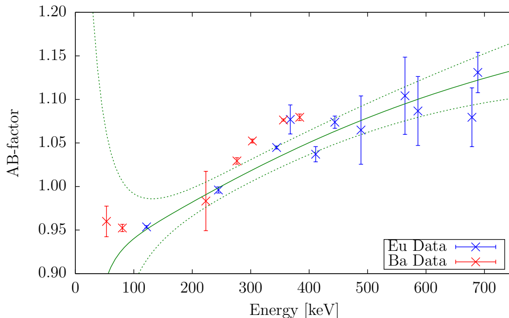
Figure 3.9: Ratio of Miniball efficiency with and without add-back. Data points are the ratios of the efficiencies of \gamma -decay lines from the ^{152}\text{Eu} and ^{133}\text{Ba} sources while the line shows the ratio of the two fitted efficiency curves shown in Figures 3.7 and 3.8 and is not a fit to the data itself. Please note that the error on this ratio becomes very large at low energies.
