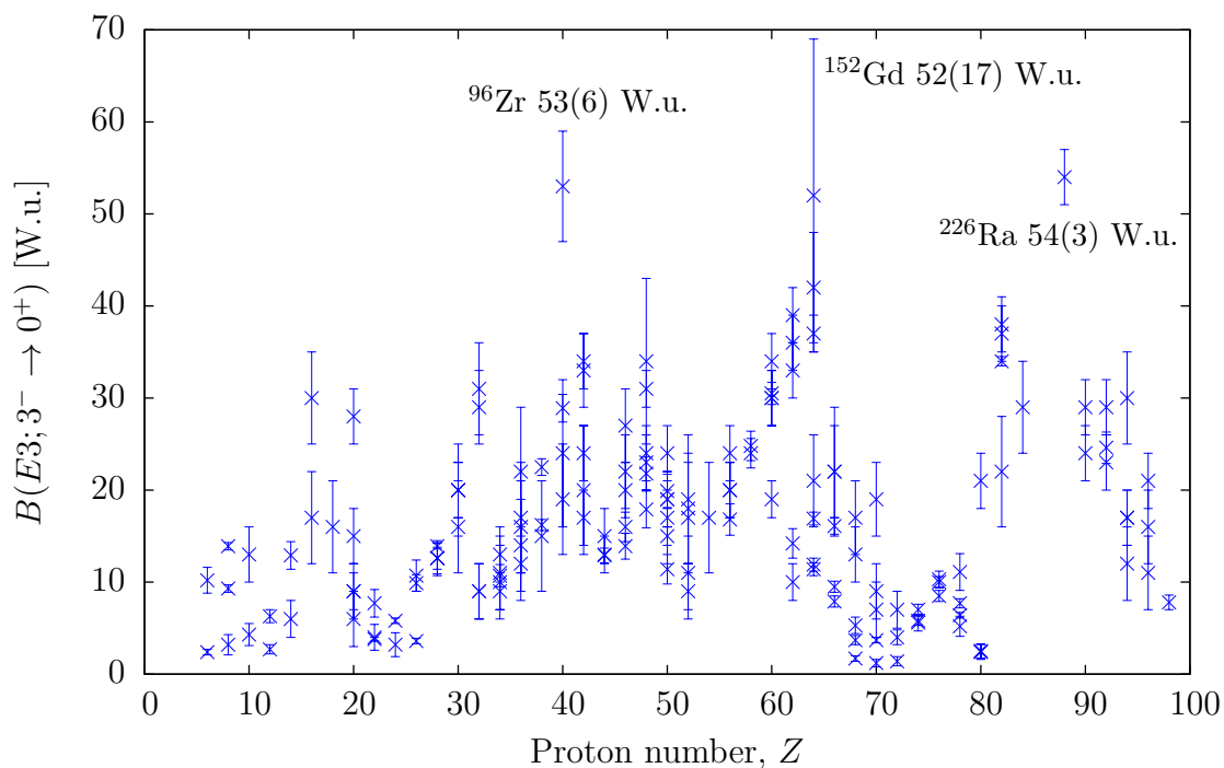
Figure 1.3: Previously measured B(E3; 3^- \rightarrow 0^+) values as a function of proton number, Z . Values are calculated from tabulated data in Ref. [30].
