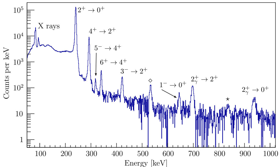
Figure 4.7: Gamma-ray spectrum of particle- gamma singles events in ^{220}\text{Rn} , Doppler corrected and background subtracted. Transitions labeled were either previously observed or determined in this work (see Section 4.2.1). The 534 keV peak, labelled with a diamond ( \diamond ), is a sum peak caused by the pileup of the 241 keV, 2^+ \rightarrow 0^+ and 293 keV, 4^+ \rightarrow 2^+ transitions. The 836(2) keV peak, labelled with a star ( \star ), is unplaced in this nucleus. Data from Sn and Ni target experiments are summed but the Cd data is not included for clarity of presentation.
