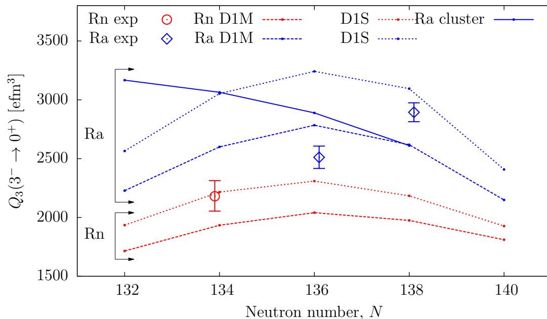
Figure 6.5: Comparison of experimental Q_3(3^- \rightarrow 0^+) from Table 6.1 for Rn ( Z = 86 ) and Ra ( Z = 88 ), with predictions from two different models overlaid. The solid lines join the cluster model predictions of Shneidman et. al [113]. The dashed lines connect points predicted by the mean-field calculations using the generator-coordinate extension (GCM) of the HFB theory with Gogny forces by Robledo and Bertsch [109]. Two parameterisations are compared, D1M and D1S.
