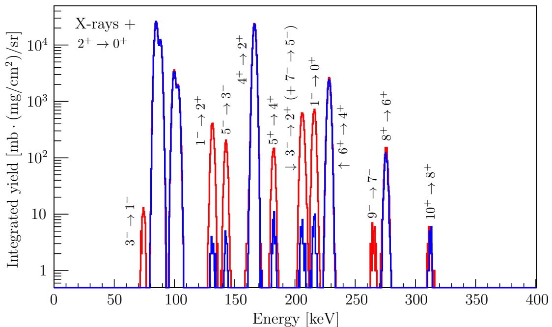
Figure 6.1: Comparison of simulated \gamma -ray yields in ^{224}\text{Ra} , experiment 2 (see Table 5.1), calculated using the measured matrix elements from Table 5.6 (red) and those same matrix elements, but with all E3 matrix elements equal to 0 \text{ efm}^3 (blue).
