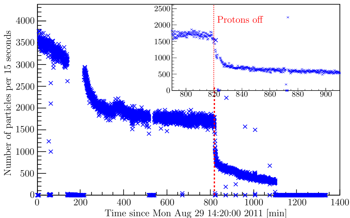
Figure 3.1: Rate of particles incident on the CD detector during and after protons were impinged on the primary target. The average current of the 1.4 GeV protons was 1.4 \mu\text{A} before the target was taken “off-line”.
