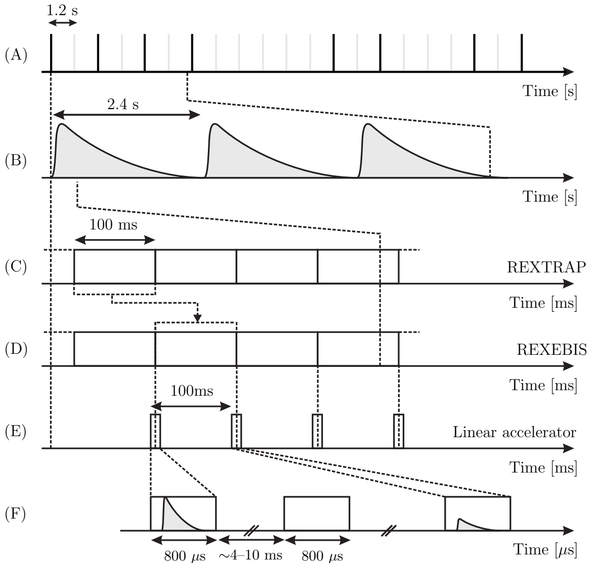
Figure 3.3: Schematic of the specific timing at ISOLDE. (A) The supercycle of proton bunches of \approx 100 \mu\text{s} width from CERN’s PS Booster separated by 1.2 seconds. The ISOLDE primary target receives an allocation of the bunches, shown in black, while others in the supercycle are distributed to other experiments. (B) Release profile of produced isotopes from the primary target. The release curves of ^{220}\text{Rn} and ^{224}\text{Ra} will be very different due to the varying half-lives and ionisation mode. (C-D) REXTRAP and REXEBIS beam bunches, synchronised with (E) the RF window of the REX linac. (F) The 800 \mu\text{s} “on-beam” and “off-beam” time windows using the Miniball setup.
